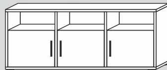
60232/40/F/G* 134x54x40cm (BxHxT) 60232/32/F/G* 134x54x32cm (BxHxT)
