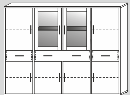
60667/40/F/G* 178x134x40cm (BxHxT) 60667/32/F/G* 178x134x32cm (BxHxT)
