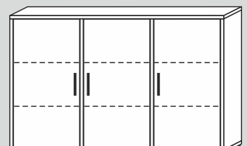
60294L/40/F/G* 134x86x40cm (BxHxT) 60294L/32/F/G* 134x86x32cm (BxHxT)
