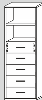
60521L/40/F/G* 46x134x40cm (BxHxT) 60521L/32/F/G* 46x134x32cm (BxHxT)
