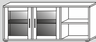
60228L/40/F/G* 134x54x40cm (BxHxT) 60228L/32/F/G* 134x54x32cm (BxHxT)
