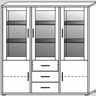
60622L/40/F/G* 134x134x40cm (BxHxT) 60622L/32/F/G* 134x134x32cm (BxHxT)
