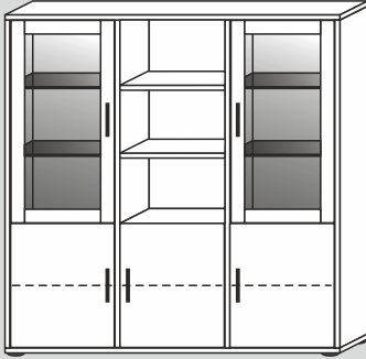
60626/40/F/G* 134x134x40cm (BxHxT) 60626/32/F/G* 134x134x32cm (BxHxT)
