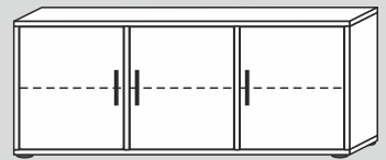
60238L/40/F/G* 134x54x40cm (BxHxT) 60238L/32/F/G* 134x54x32cm (BxHxT)
