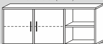
60227L/40/F/G* 134x54x40cm (BxHxT) 60227L/32/F/G* 134x54x32cm (BxHxT)
