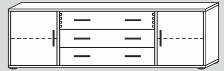
60357/40/F/G* 178x54x40cm (BxHxT) 60357/32/F/G* 178x54x32cm (BxHxT)
