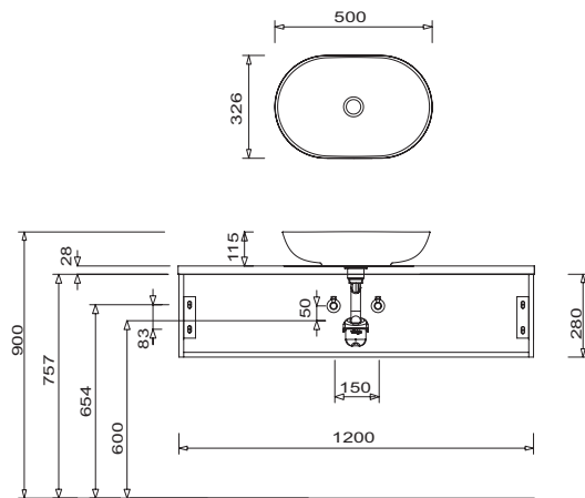
WSA 3250 41 + APA 4512 28 + WUA 1212 G6
