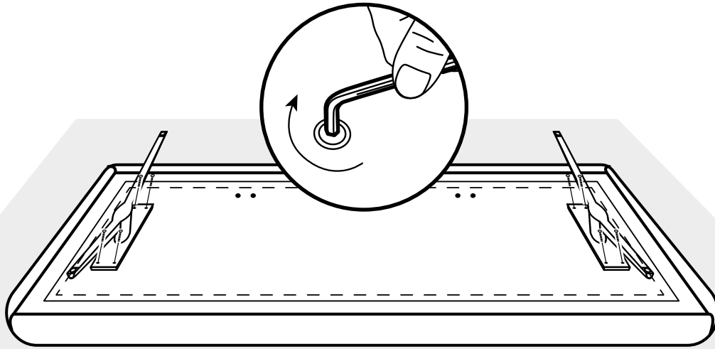
Schwertkufe Aluminium casting sword runner
