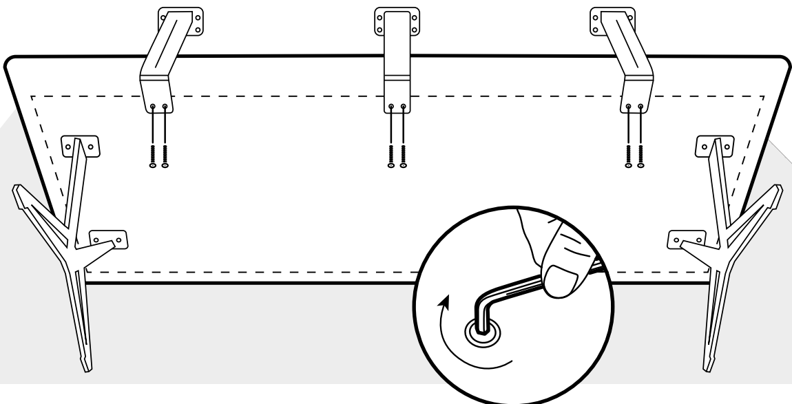
Senkkopfschraube 8x30 mm Countersunk head screw 8x30 mm
